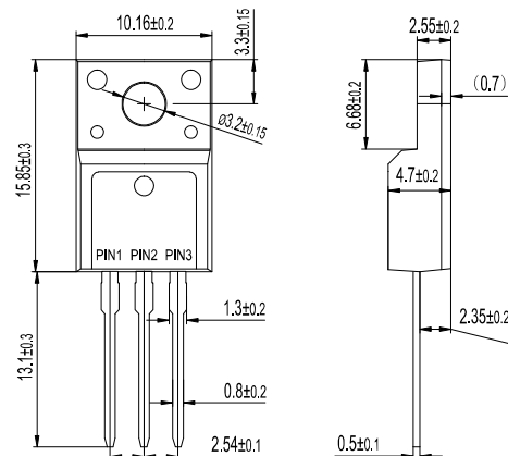
ITO-220AB FR20XXFCT
